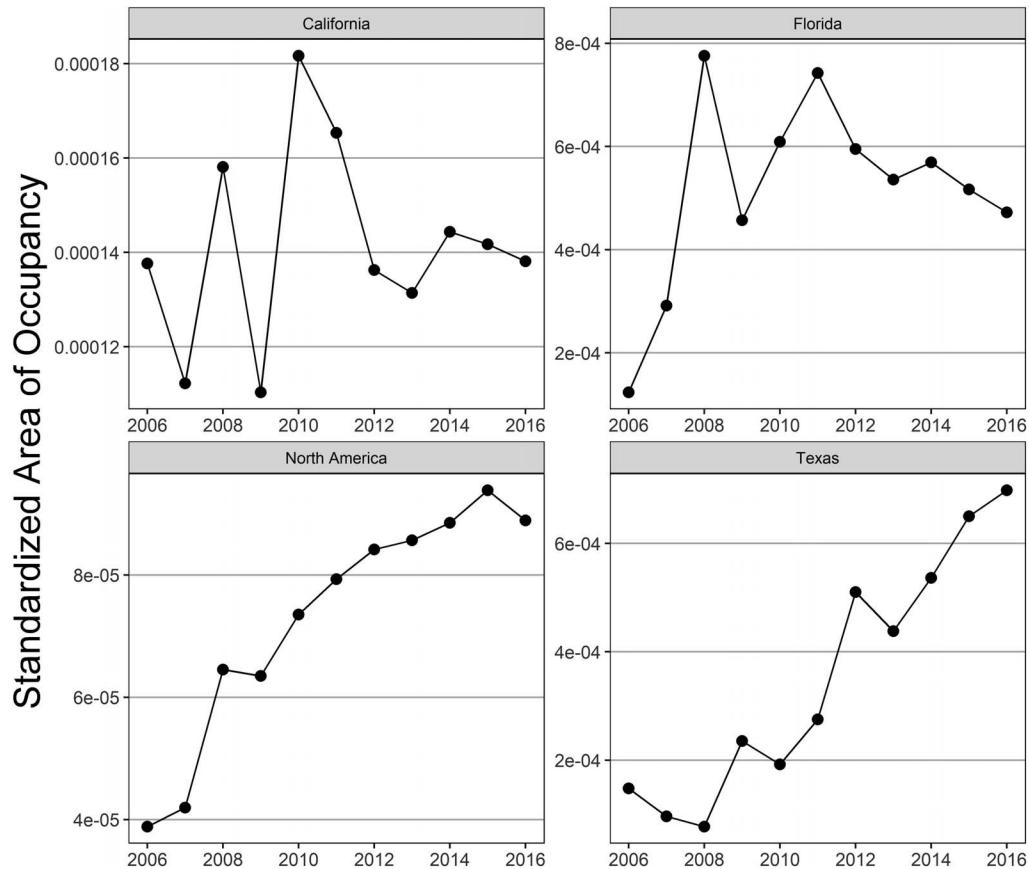
FIG. 2—The standardized area of occupancy of Egyptian geese in the contiguous United States 2006–2016. The y axis represents the area of occupancy (i.e., the number of 10-km 2 grid cells occupied in a given year) divided by the number of checklists in that given geographic location (as a measure of effort). Note the different y axes scales, which reflect the different number of checklists used to standardize the data, in order to account for effort.
