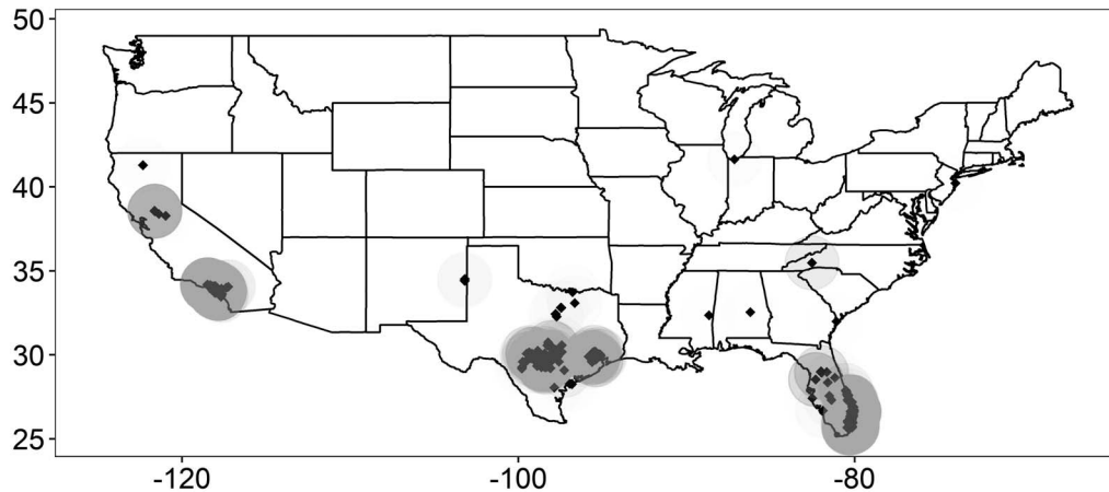
FIG. 1—The current distribution of the Egyptian goose throughout the continental United States. Maps are made using Program R statistical software, eBird data from January 2016 to December 2016 ( N = 2,221 observations). Each eBird occurrence during this time frame is plotted, using a “jitter” approach, which introduces a small amount of variation to the points to avoid overplotting. The circle represents the “jittering.” Minimal transparency indicates minimal points plotted on top of each other, while the darker areas indicate many points plotted on top of each other.
